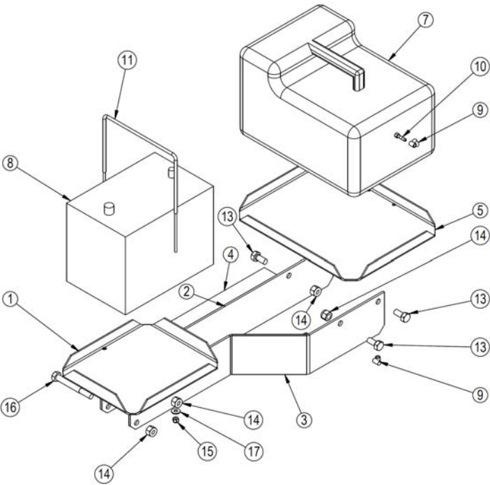
TANK ASSEMBLY
