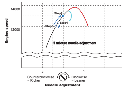
Fig. 2: WOT setting
