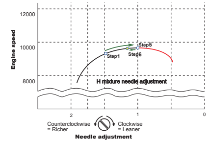
Fig. 3: WOT setting
