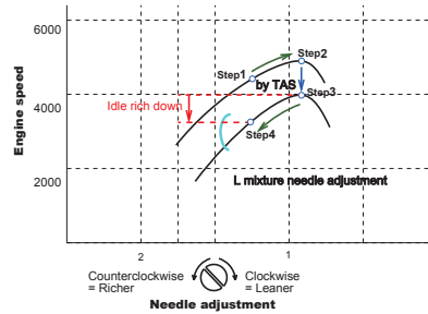
Fig. 1: Idle setting
