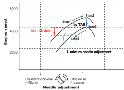
Fig. 1: Idle setting
