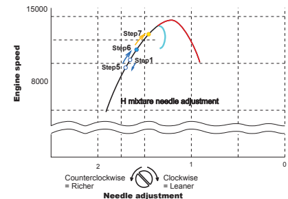
Fig. 4: WOT setting
