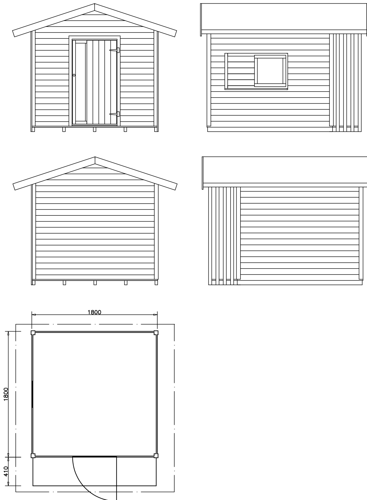
Playhouse 30 / Satakieli: 1800 x 1800 mm (410 mm) / 16 mm
