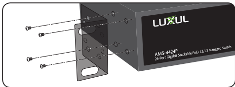
Rack-Mounting the AMS-4424P
