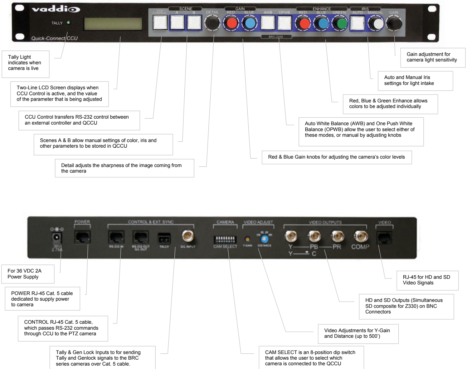
Figure 2: Quick-Connect CCU interface front panel and rear panel diagrams with functional callouts.
