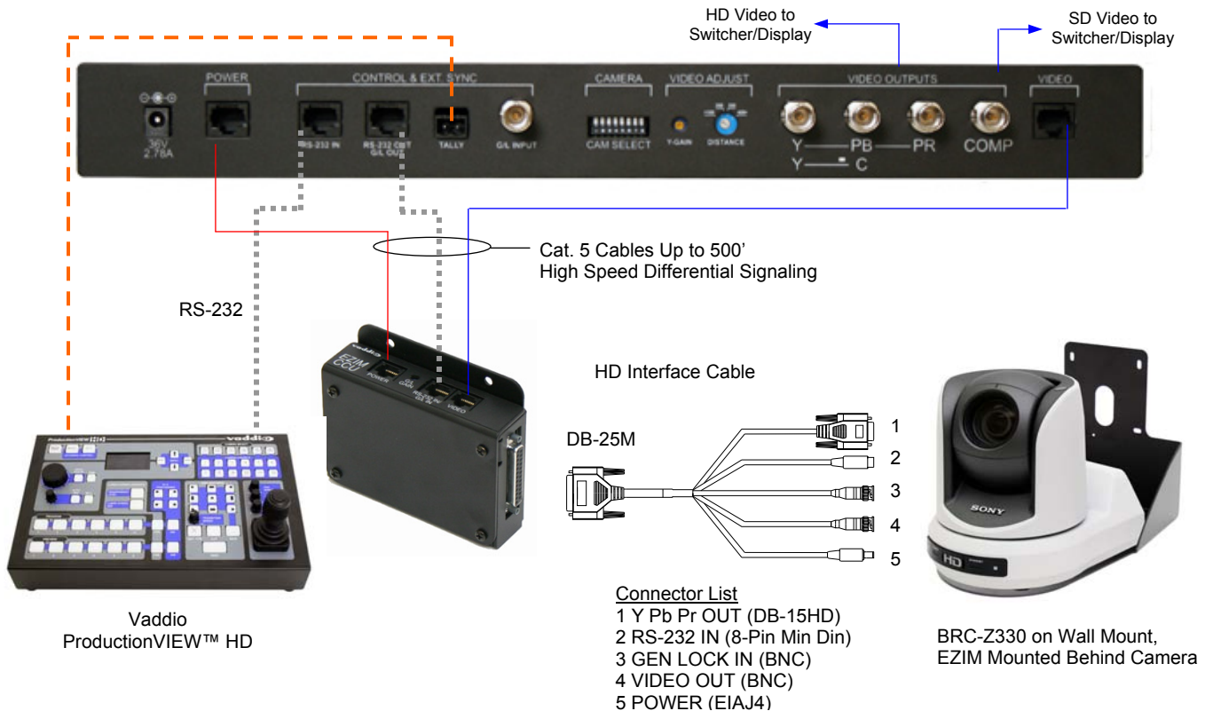
Figure 4: Basic system connectivity of a WallVIEW CCU Z330 System and ProductionVIEW Super Joystick Controller
