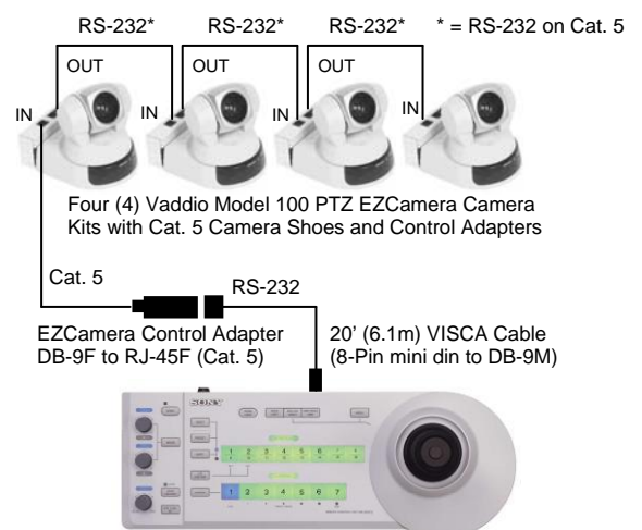
Figure 2: Sony RM-BR300 Joystick with Daisy Chain Control
