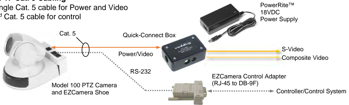
Figure 2: Multi-Camera Control (daisy-chaining control):
