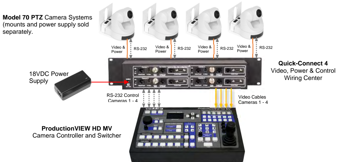
Figure 3: Multi-Camera EZCamera System with Vaddio ProductionVIEW™ and Quick-Connect™ 4
