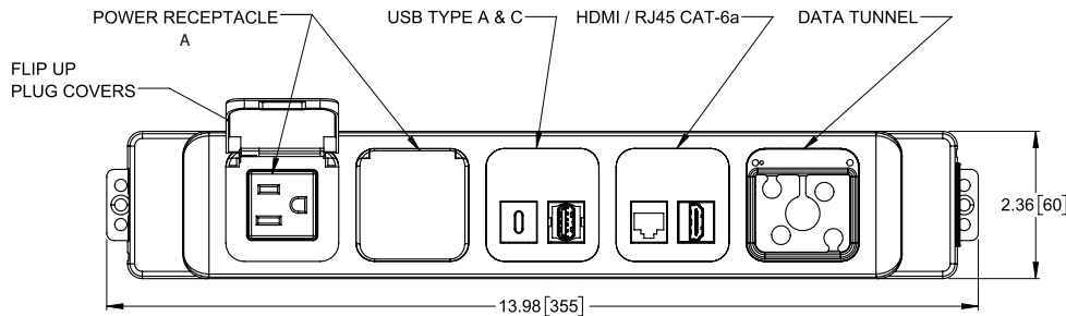
SIMILAR CONFIGURATION FOR BOTH NETBOX M AND AXIAL MODELS SCALE: 1/2
