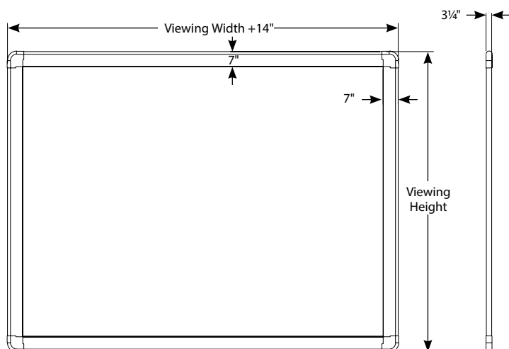
Frame Shown Assembled With Pro-Trim® Masking Cover
