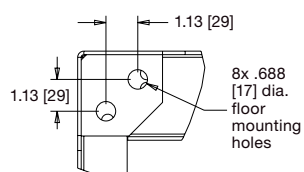
detail A for DRK, MRK, WRK, VRK Series
