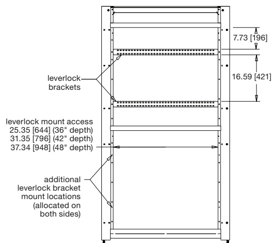
cable chase side view (without side panels)
