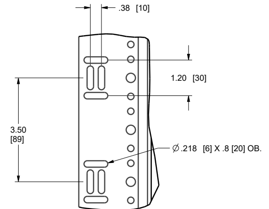
DETAIL C SCALE 1/2 REAR RACKRAIL COMPATIBLE WITH ALL FORWARD CABLE MANAGEMENT ACCESORIES
