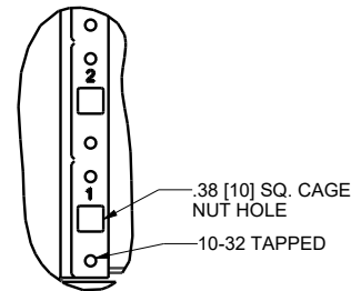
DETAIL D SCALE 1/2 FORWARD COMPATIBLE RACKRAIL
