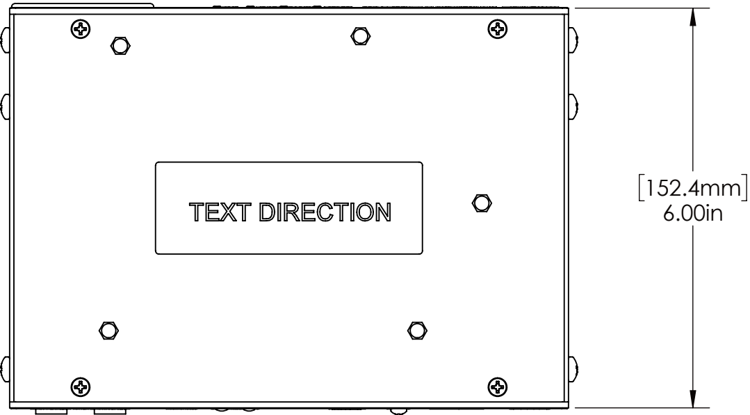
BOTTOM VIEW
