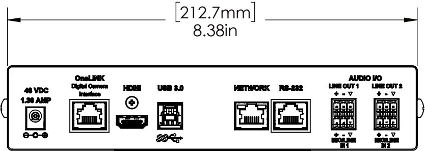
REAR VIEW
