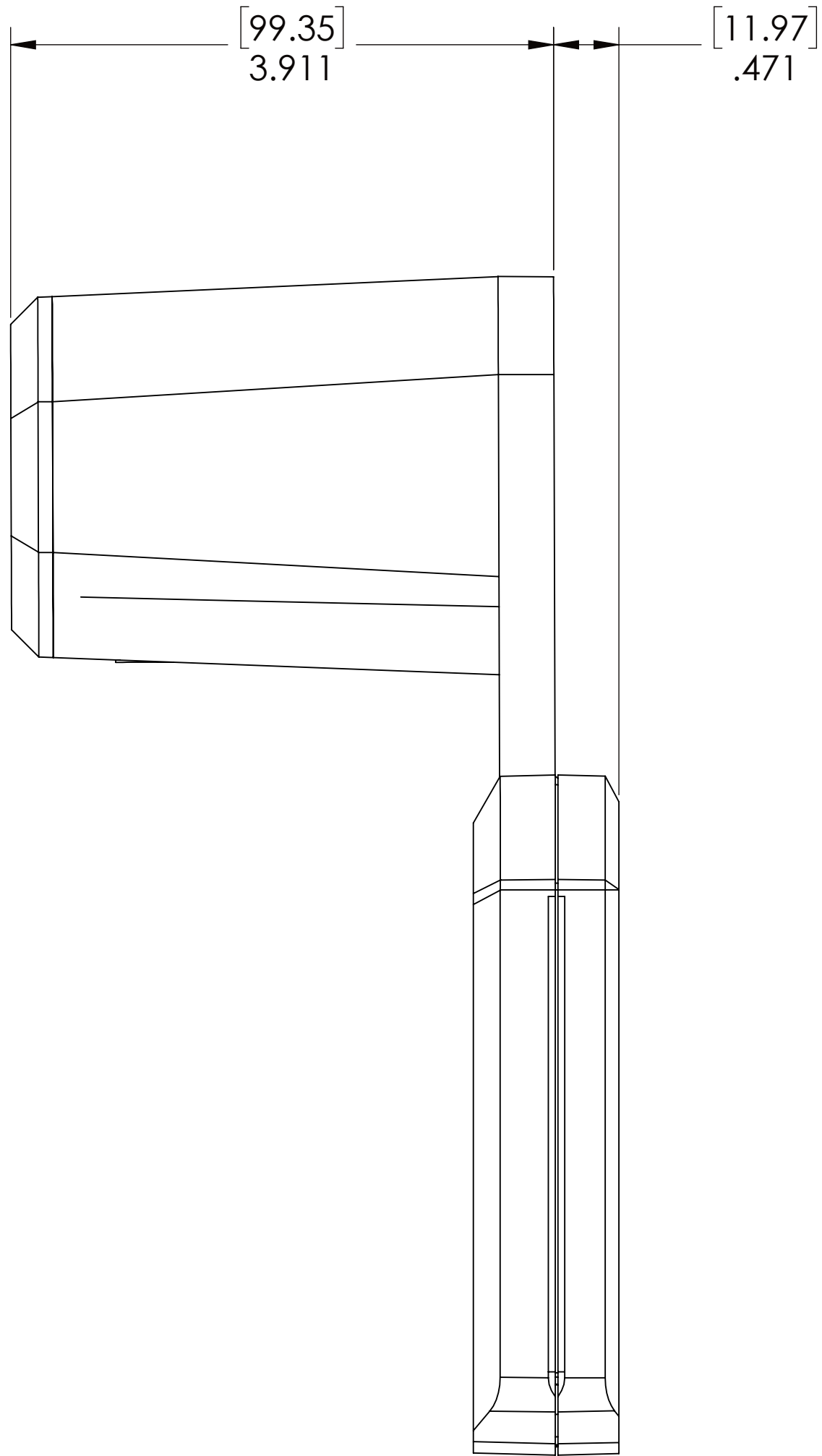
SIDE VIEW 2
