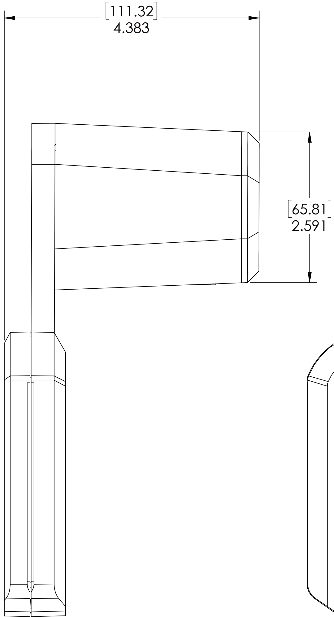
SIDE VIEW 1
