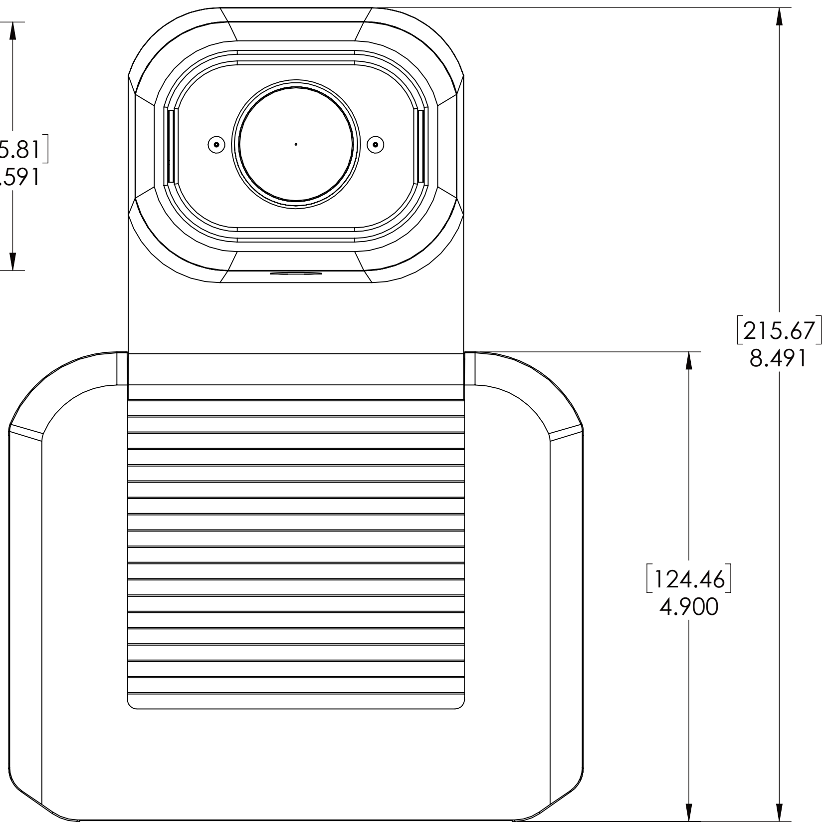
FRONT VIEW
