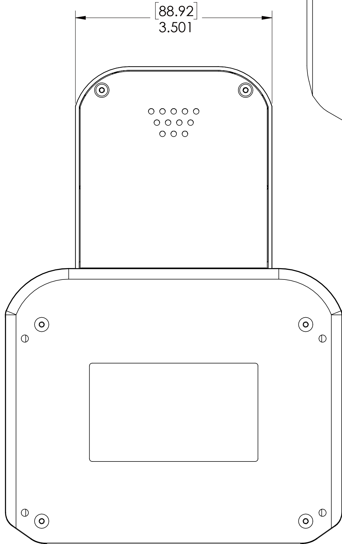
REAR VIEW
