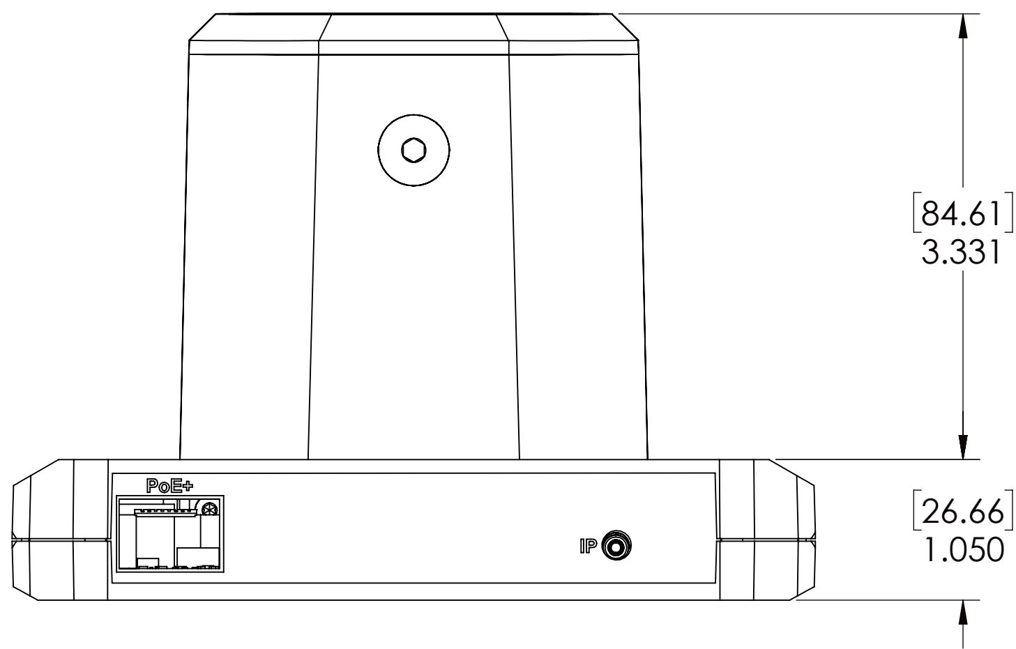
FRONT VIEW
