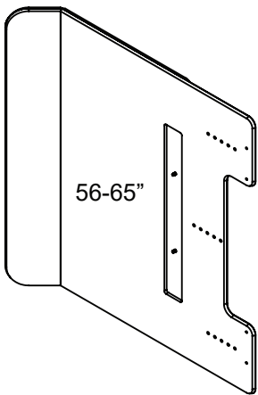
Shroud Pairs NOTE: Left shroud is shown for a 56-65" Dual Display. L
