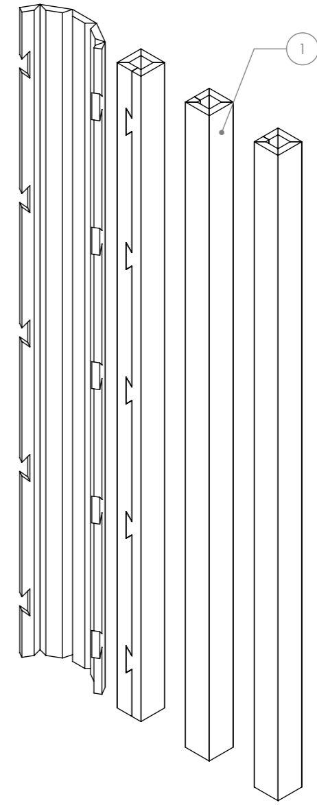
EXPLODED
