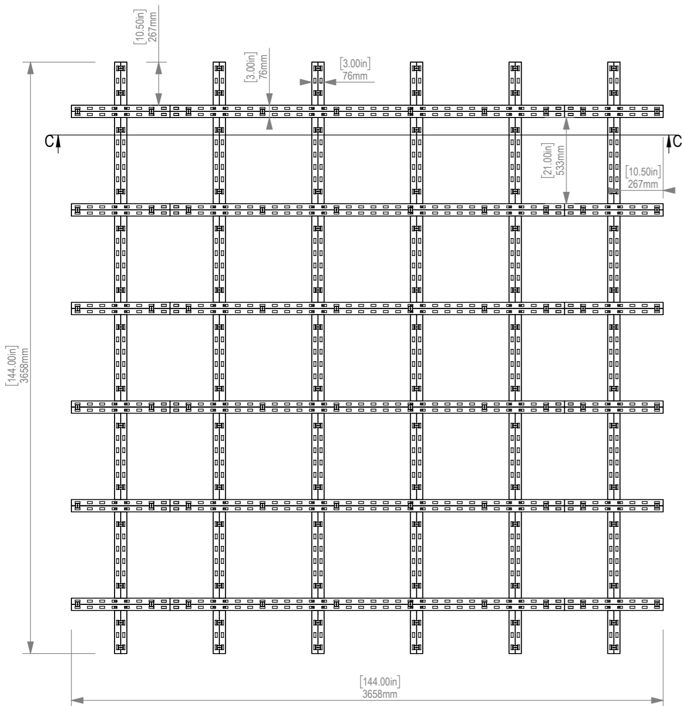
TOP VIEW
