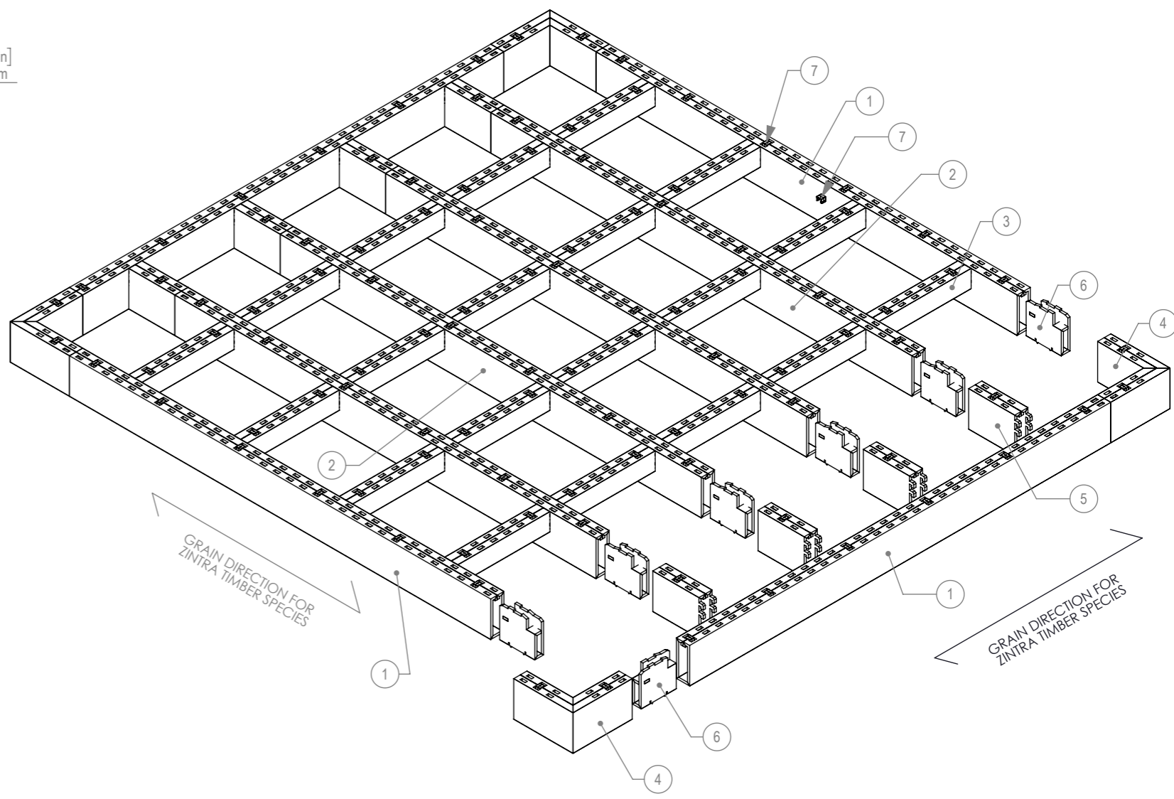
EXPLODED
