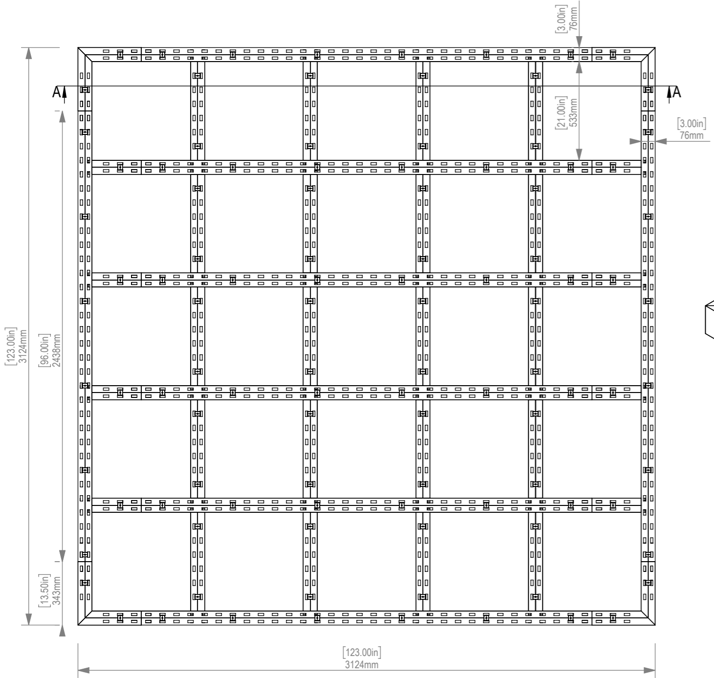
TOP VIEW
