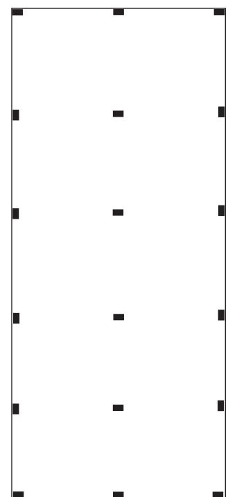
Full Sheet - 48x110in. 2800mm x 1225mm
