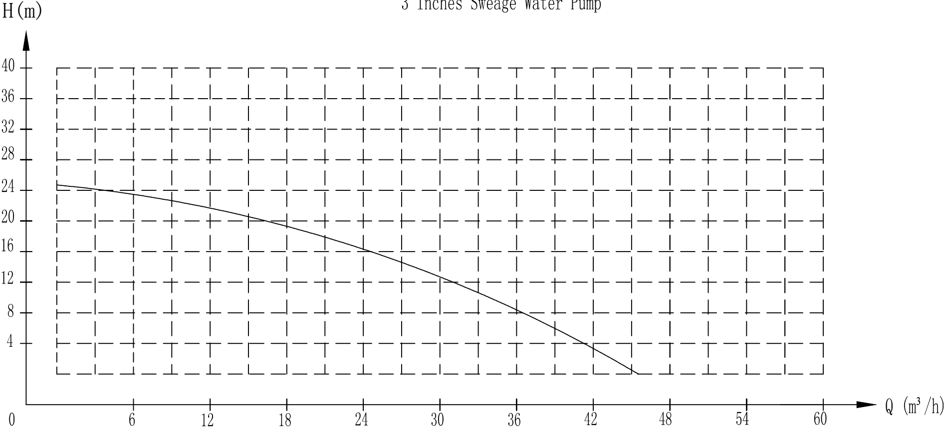
3 Inches Sweage Water Pump
