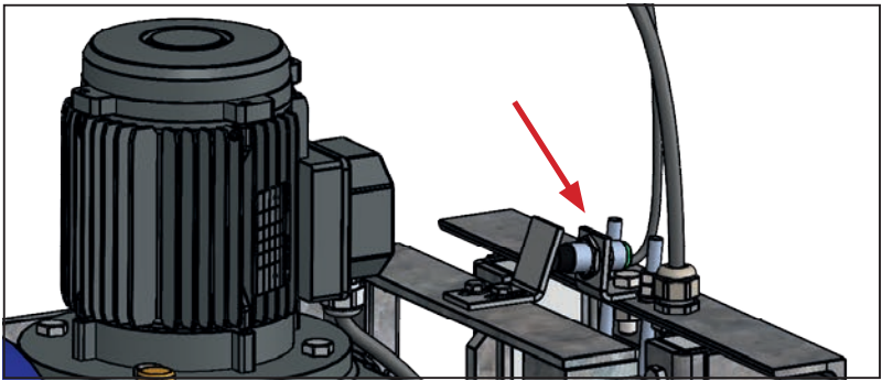
Figure 10: Mounting position of the sensor
