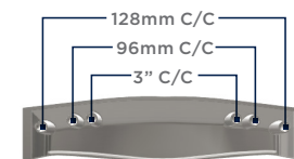
Back View
