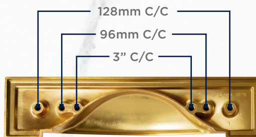
Back View
