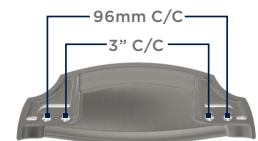
Back View
