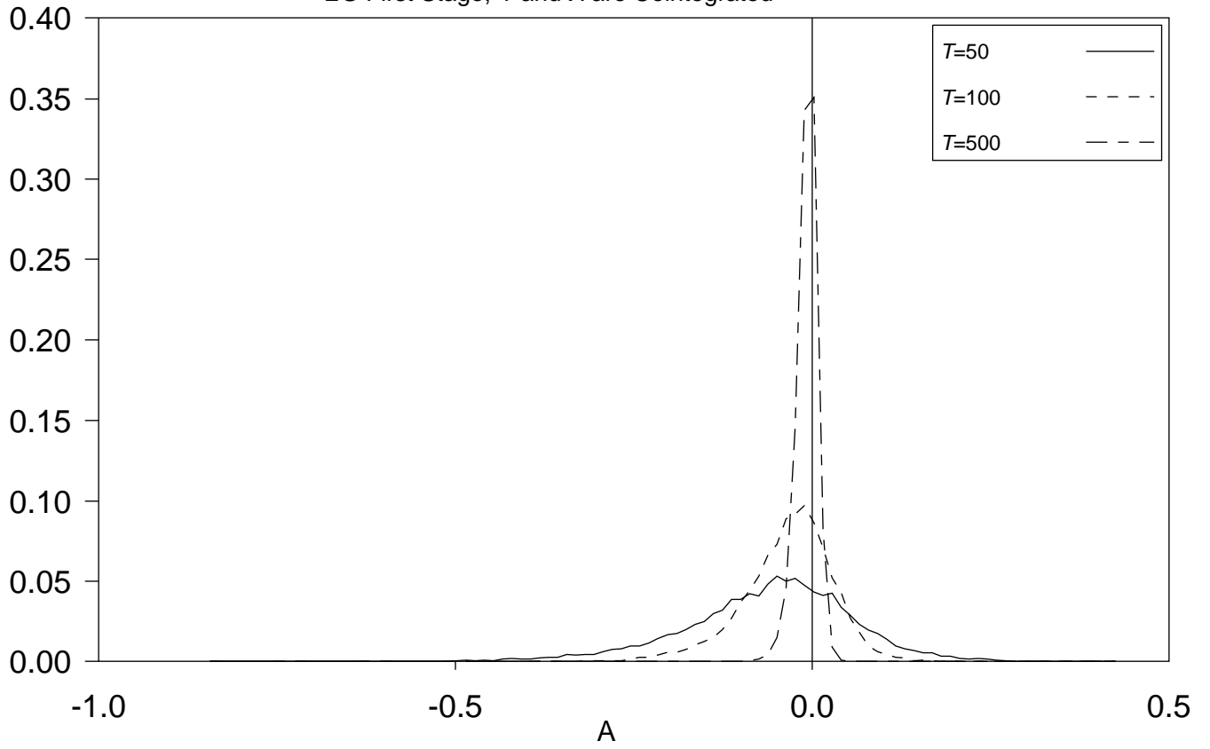
EG First Stage, Y and X are Cointegrated
