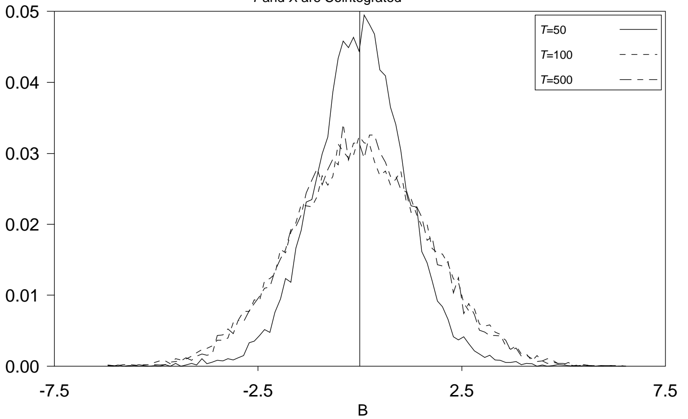
Y and X are Cointegrated
