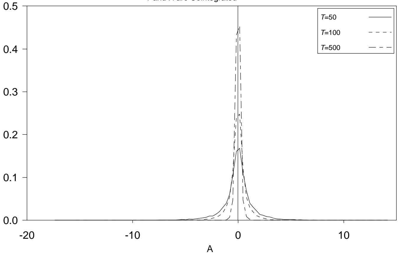
Y and X are Cointegrated
