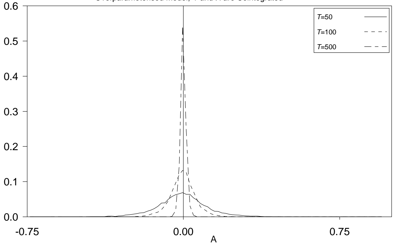
Overparameterised Model, Y and X are Cointegrated
