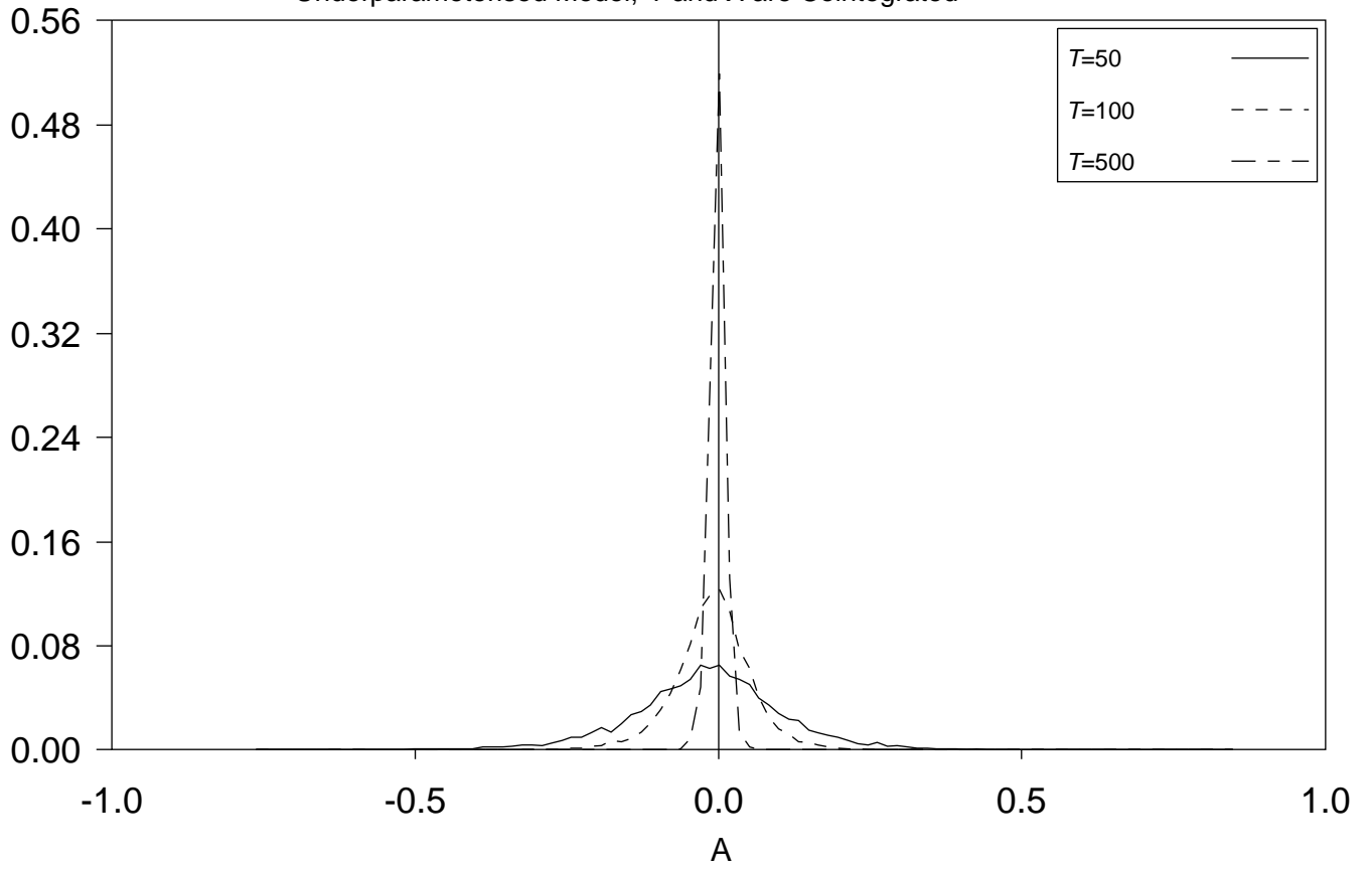
Underparameterised Model, Y and X are Cointegrated
