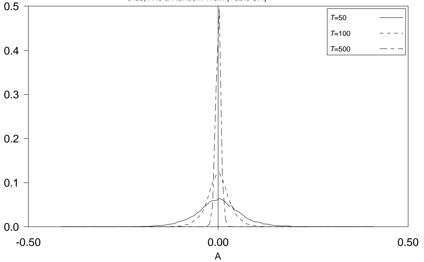
Bias, X is a Random Walk (Table 8.4)
