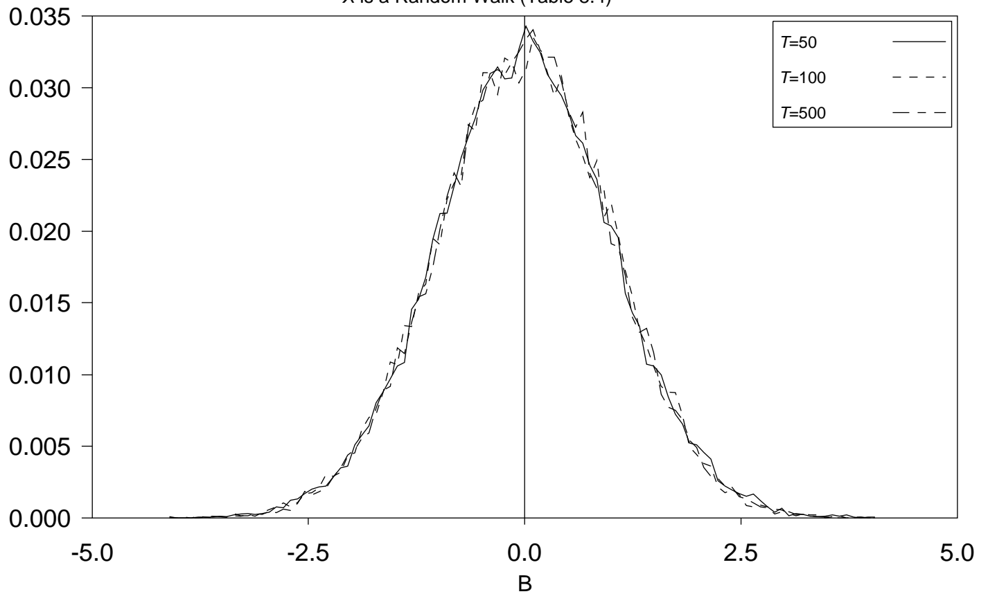
X is a Random Walk (Table 8.4)
