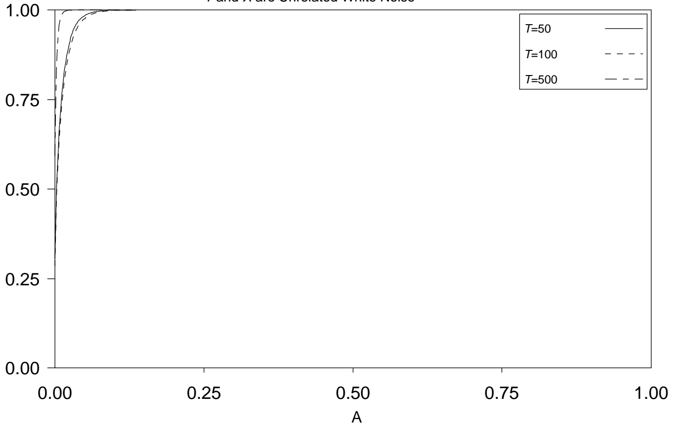
Y and X are Unrelated White Noise
