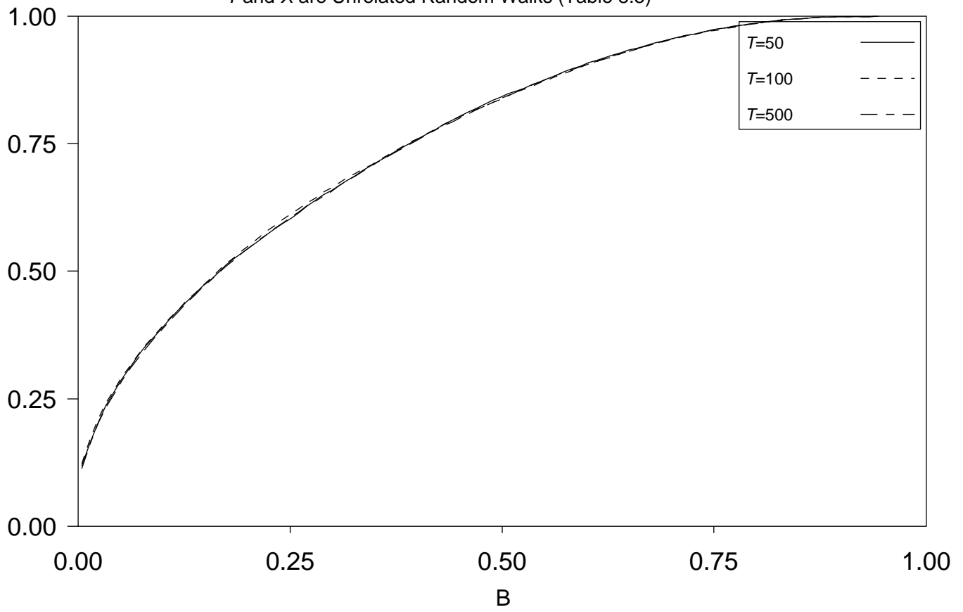
Y and X are Unrelated Random Walks (Table 8.5)
