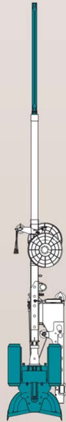
KRC DIAPHRAGM WALL Depth 30 m Trench 800 x 2500 mm
