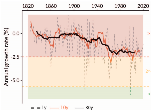
Fig. 6. Rates of growth of global carbon intensity, measured as GHGe (kg of CO 2 e) per $ of GDP ($2011): annual (grey), 10-year moving average (red), 30-year moving average (black). (For interpretation of the references to colour in this figure legend, the reader is referred to the web version of this article.)
