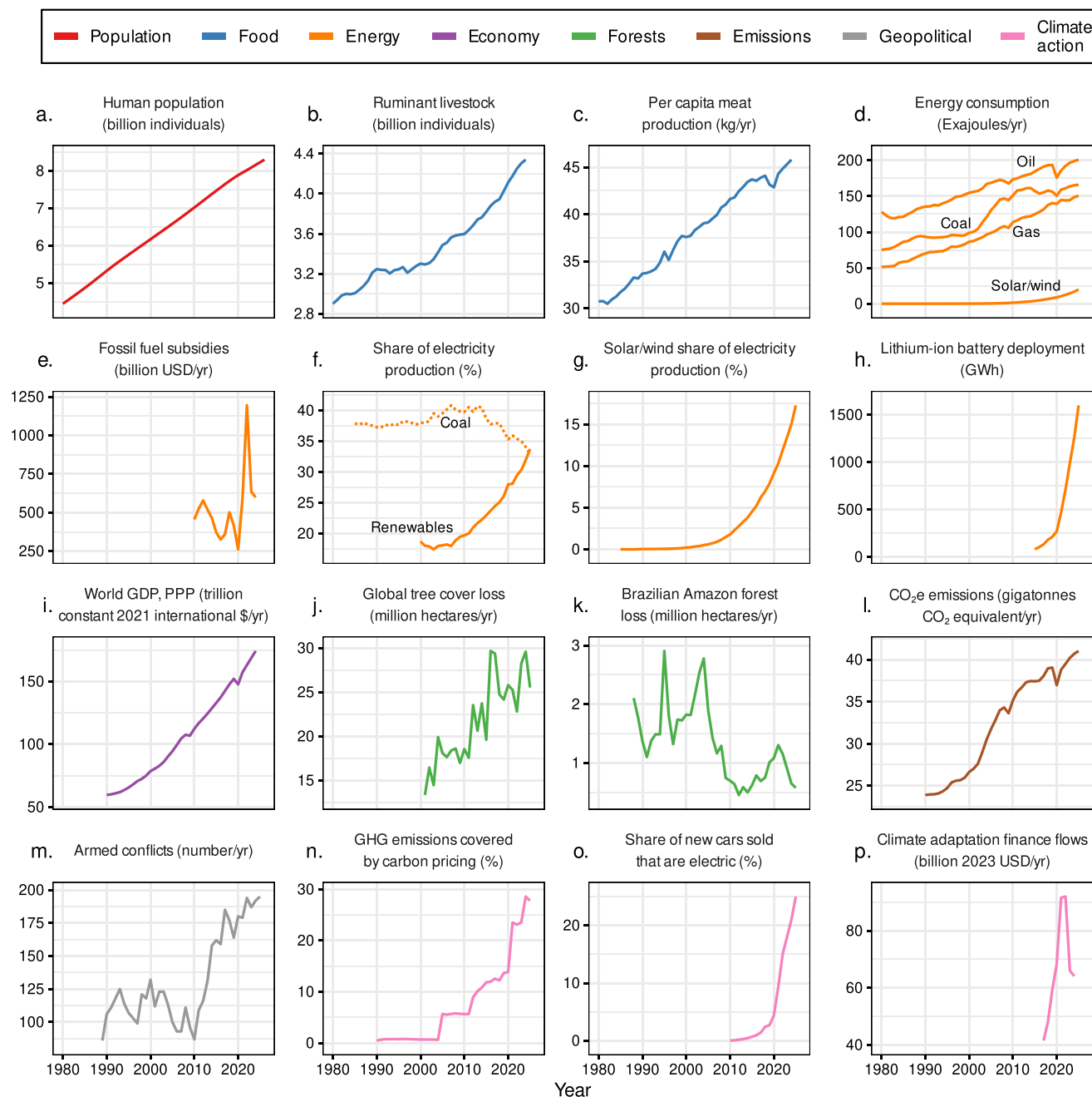
Figure 2. Time series of climate-related human activities. In panel (j), tree cover loss does not account for forest gain and includes loss due to any cause. For panel (d), statistics are based on total energy supply (The Energy Institute 2025); hydroelectricity and nuclear energy are shown in supplemental figure S4. Sources and additional details about each variable are provided in supplemental file S1.
