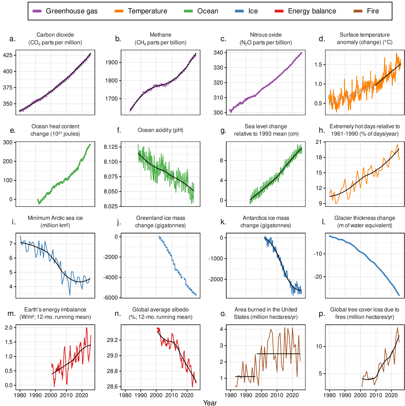
Figure 1. Time series of climate-related responses. For surface temperature anomaly (d), estimates based on a segmented linear regression model are shown in gray (prior to 2010) and black (beginning in 2010). For area burned (o), the black horizontal lines show changepoint model estimates, which indicate abrupt shifts (figure S3). For other variables with relatively high variability, local regression trendlines are shown in black. The variables were measured at various frequencies (e.g., annual, monthly, weekly). The labels on the x-axis correspond to midpoints of years. Sources and additional details about each variable are provided in supplemental file S1.
