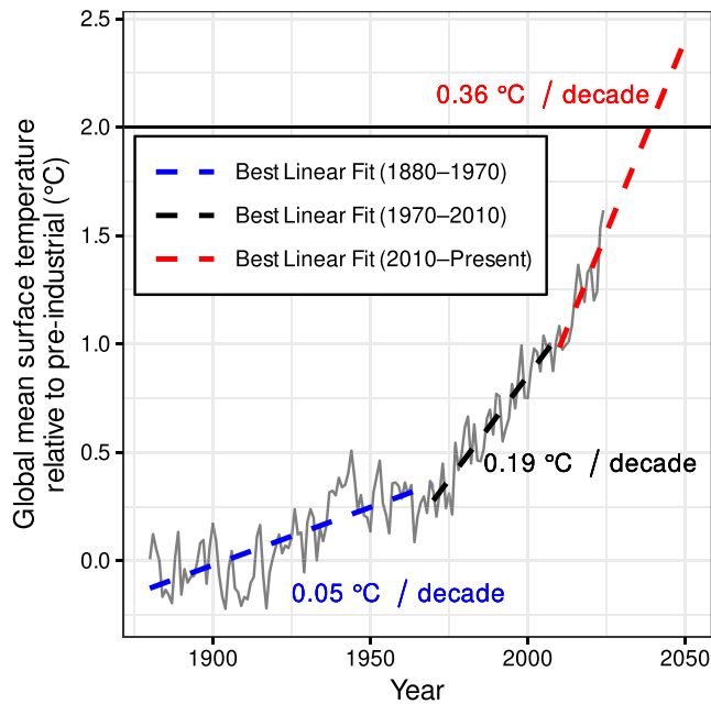
Figure 3. The rate of warming appears to be accelerating. At current rates, 2°C above pre-industrial levels could be reached before 2050. Temperature data come from Rohde and Hausfather (2020). See supplemental file S3 for details.
