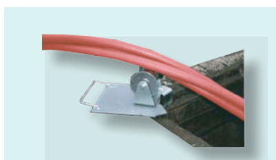
C109.E Galvanised roller guide with swivel angled base.
