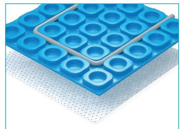
Tile decoupling heat underlayment 1m x 1m / 1m x 5m / 1m x 15m
