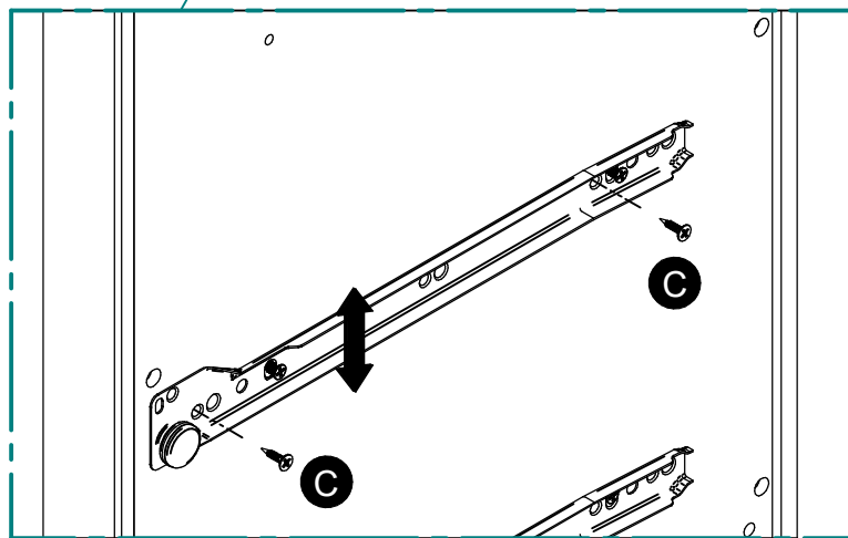
Height adjustment
