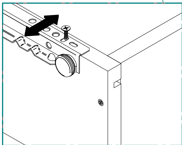
Lateral adjustment
