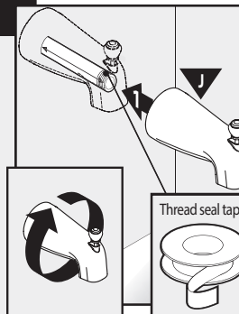
Tub Spout Installation
