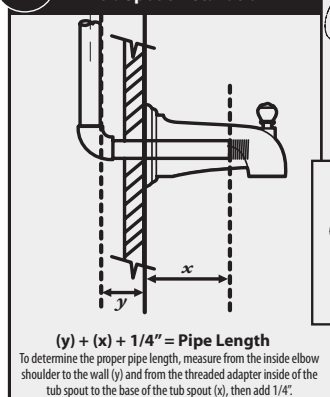
Tub Spout Installation
