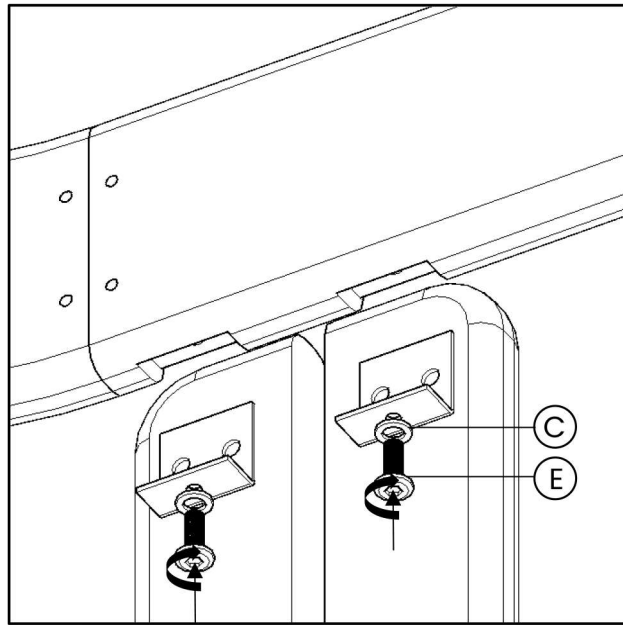
Rear legs
