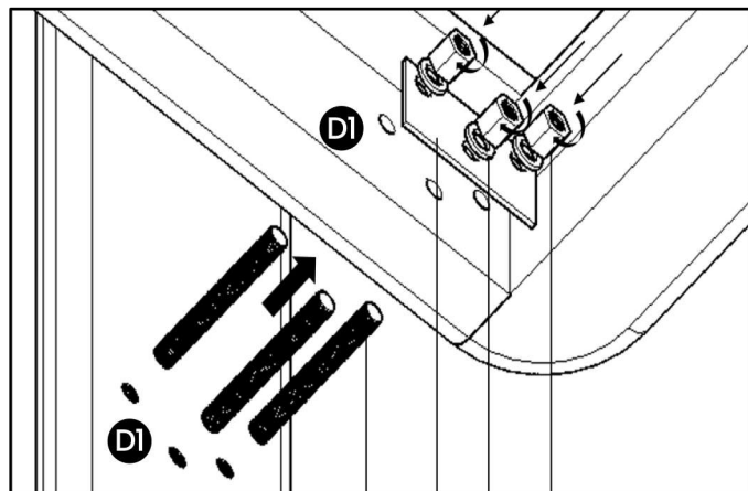
Front legs (Left)
