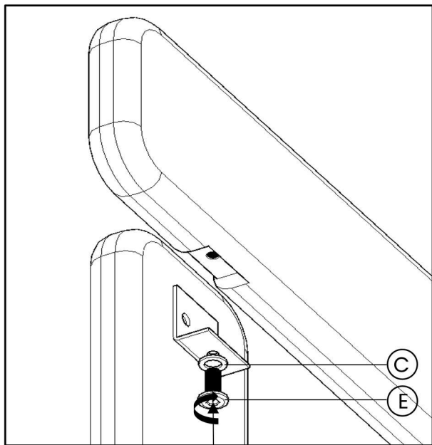
Front legs
