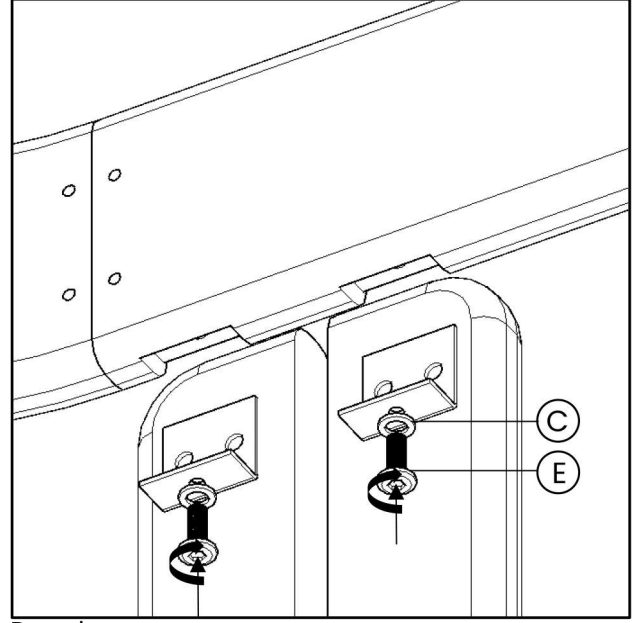
Rear legs
