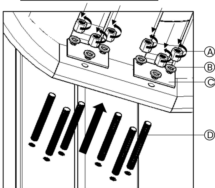
Rear leg
