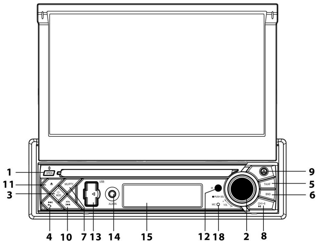
Control Panel
