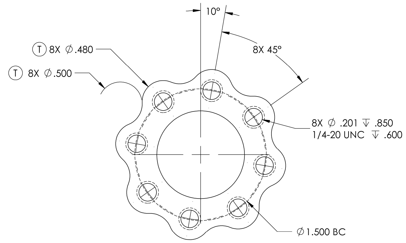
DETAIL B SCALE 3 : 2
