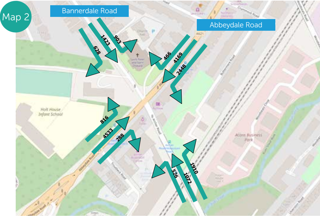
2 day average number of motor vehicles travelling through the Bannerdale Road / Abbeydale Road junction after the scheme (May 2023)
