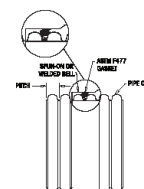
12"-60" (300-1500mm) MEGA GREEN WT IB
