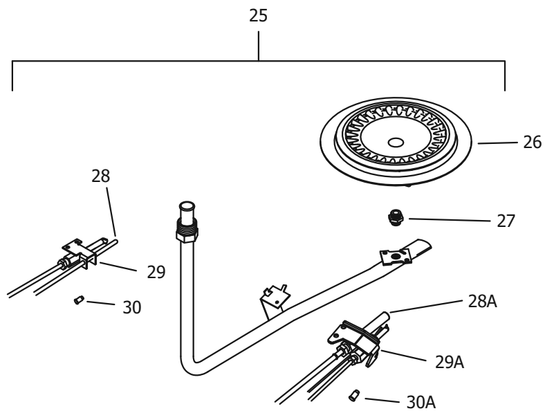
NATURAL GAS (BN) BURNER ASSEMBLY
