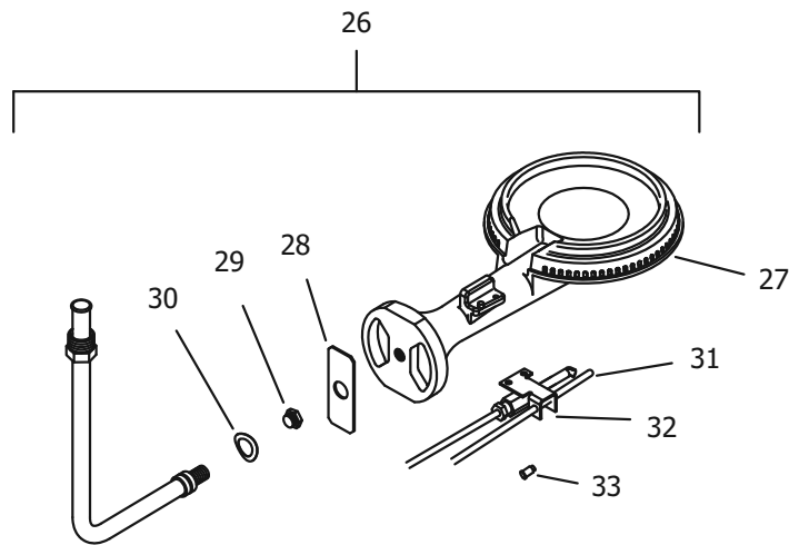
LP GAS (CX) BURNER ASSEMBLY
