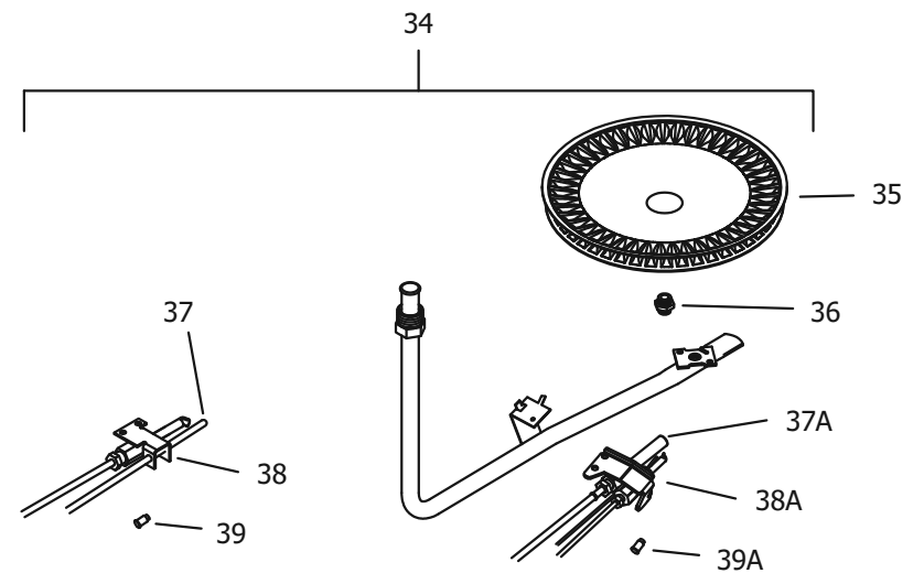
LP GAS (SX) BURNER ASSEMBLY
