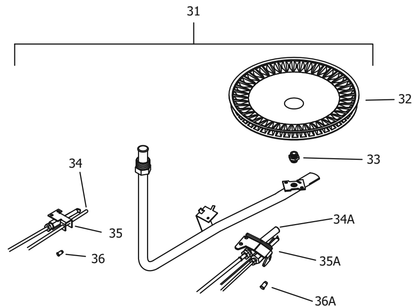
LP GAS (SX) BURNER ASSEMBLY
