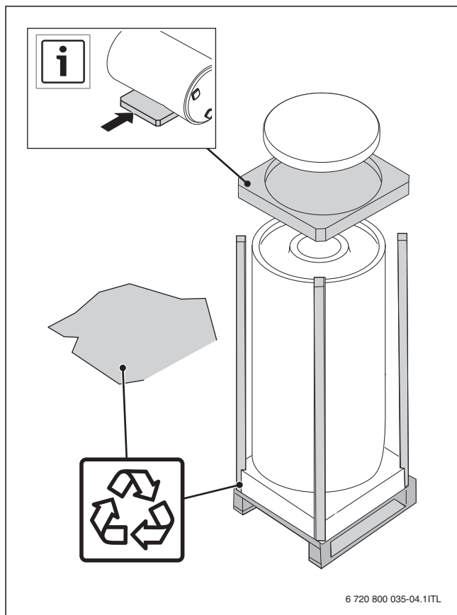
Fig. 7 Unpacking the DHW tank
