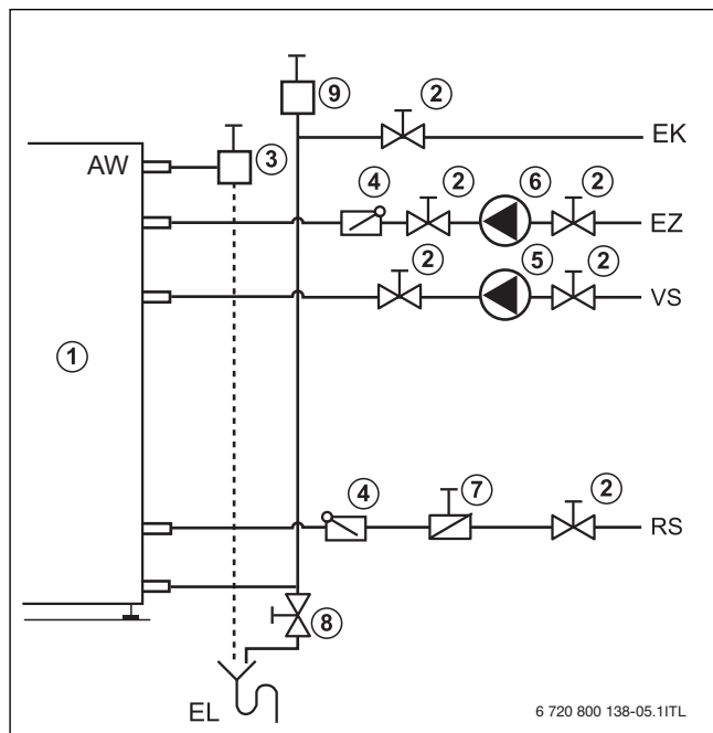
Fig. 11 Installation (illustrative)
