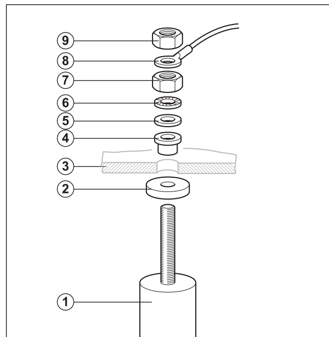
Fig. 21 Replacing the magnesium anode
