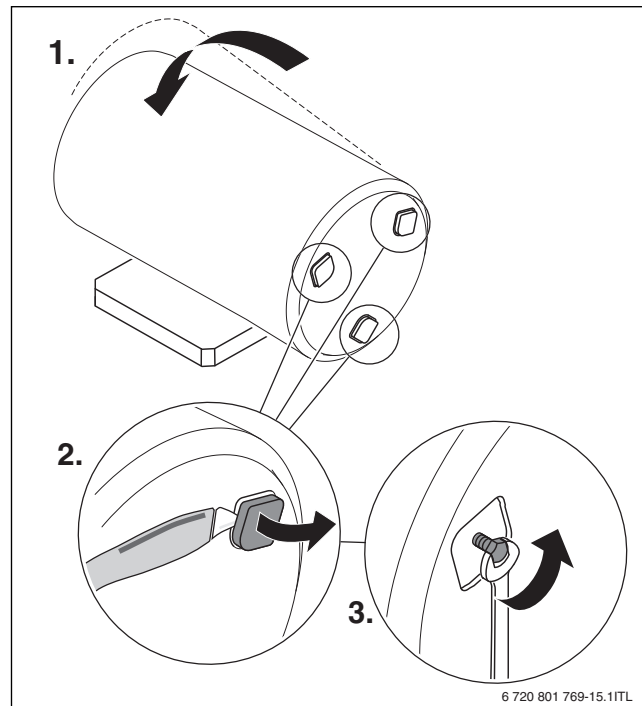
Fig. 8 Lay down the DHW tank and expose the adjustable feet
