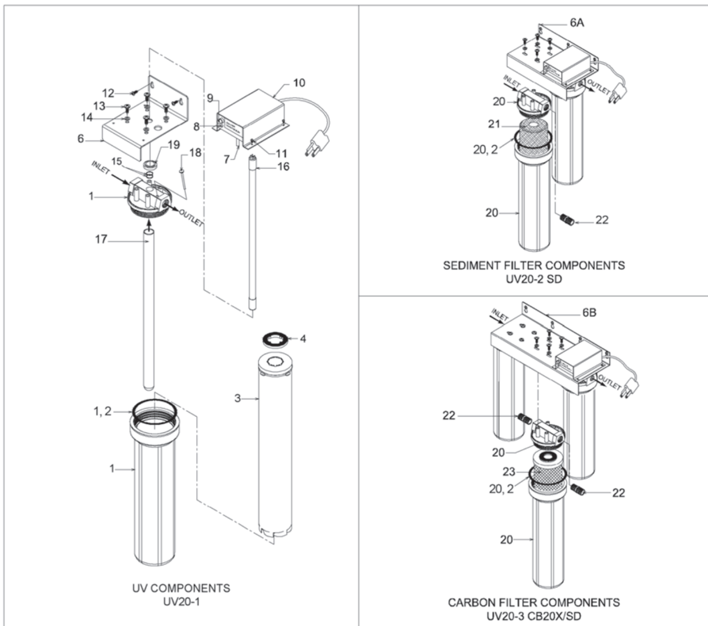
Figure 2 Exploded Schematic, PURA UV20 Series
