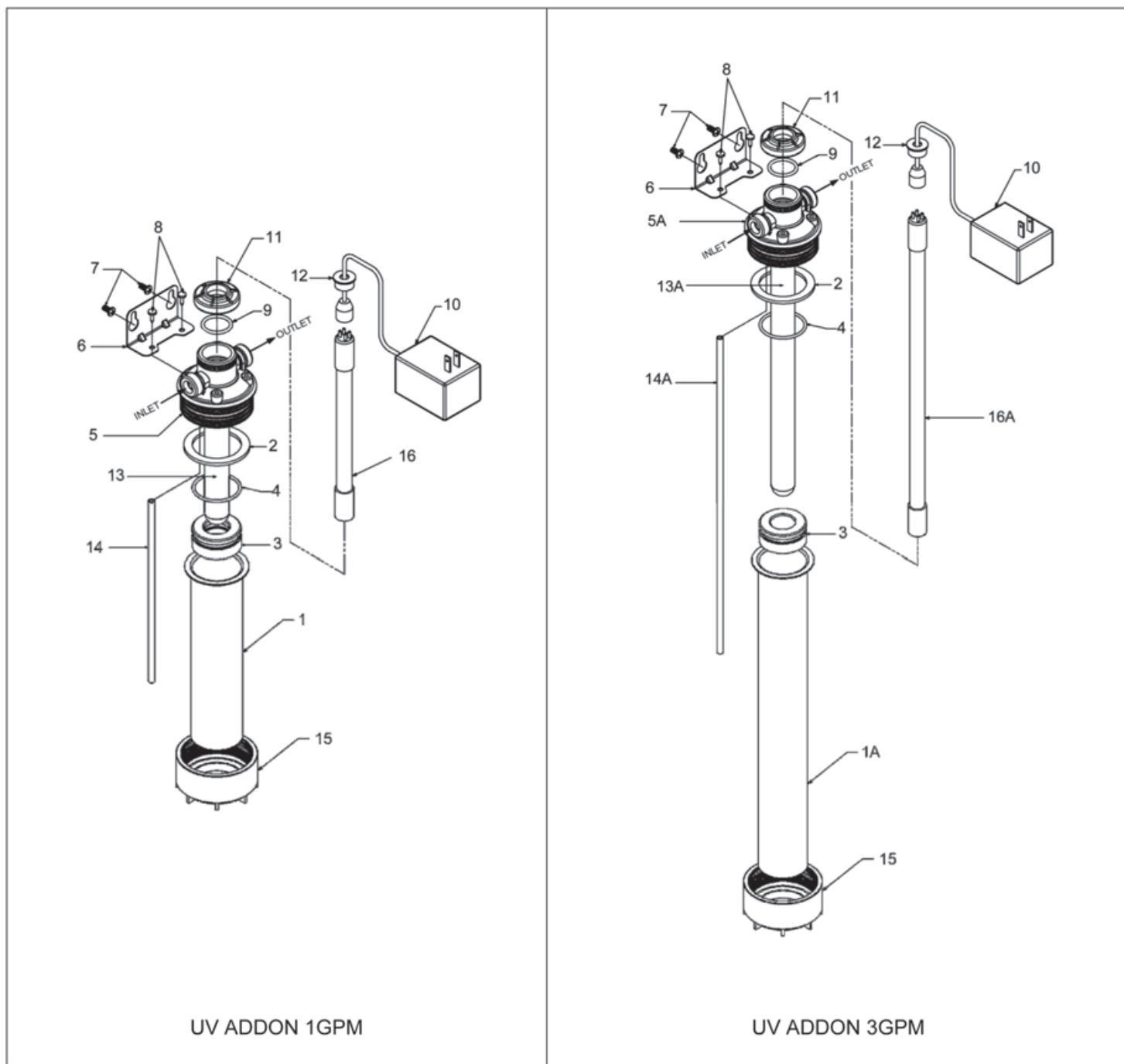
Figure 9 Exploded Schematic PURA ADDON System
