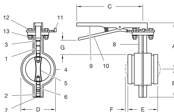
FIGURE 2 MODEL B303 BUTTERFLY VALVE WITH LEVER-LOCK OPERATORS
