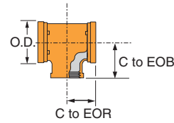
FIGURE 7065 STANDPIPE TEE (GR x GR x FPT)
