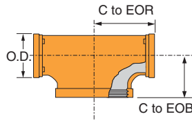
FIGURE 7062 BULLHEAD TEE (GR x GR x FPT)
