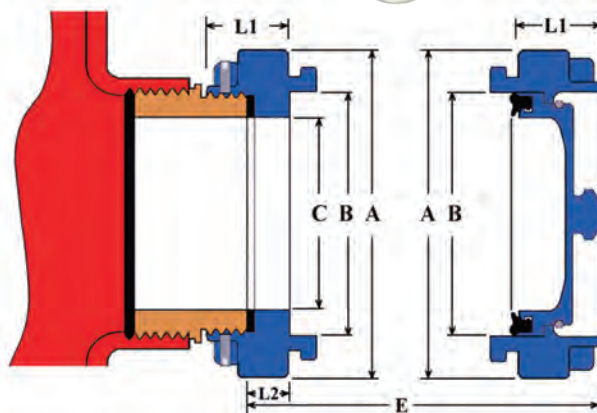
HPHA40-45NH/Cap
