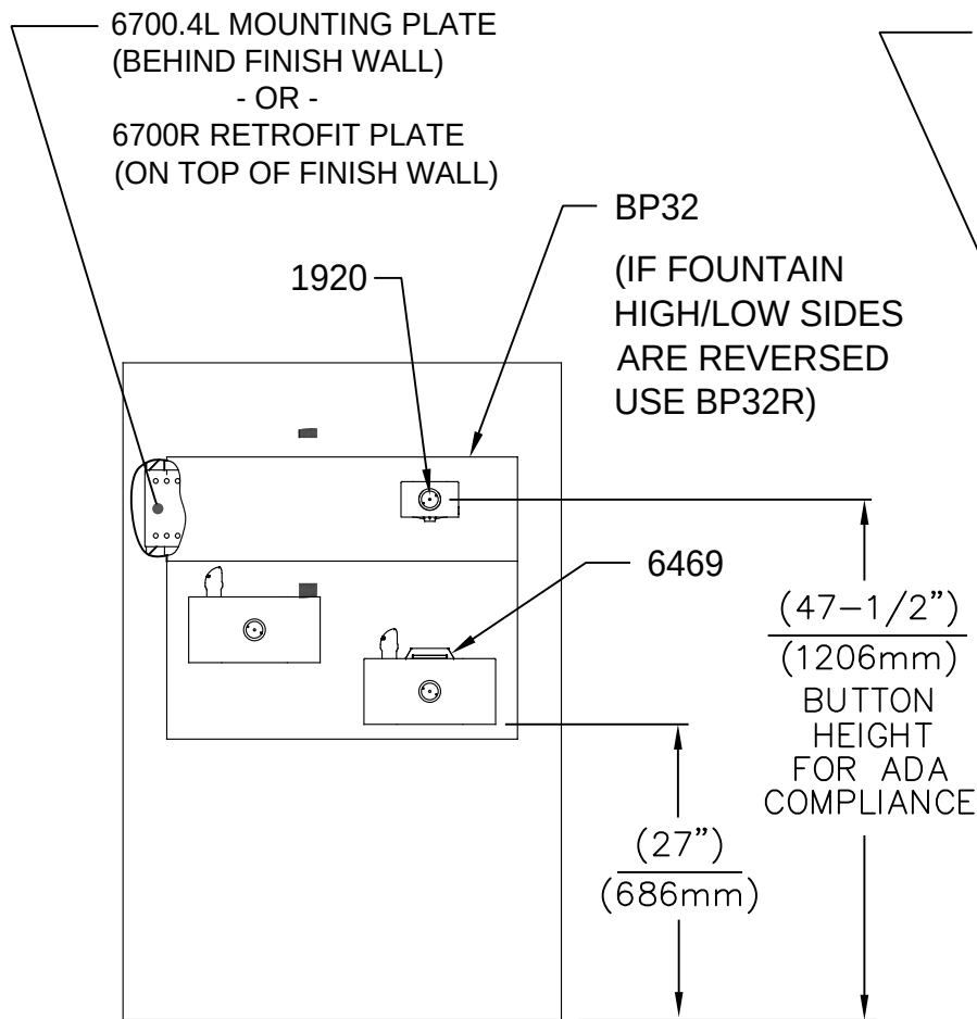
INSTALLATION ABOVE HAWS 1119, 1119.14, H1119.8
