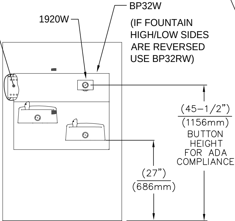
INSTALLATION ABOVE HAWS 1501
