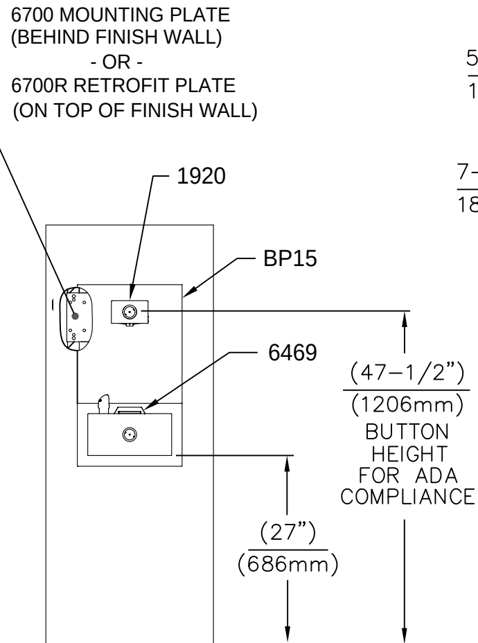
INSTALLATION ABOVE HAWS 1109, 1109.14, H1109.8
