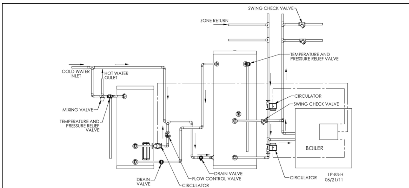
Figure 7 - Installation with Storage Tank
